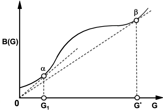
(a) Two Multiple Tangents.
