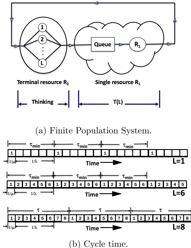
Figure 4: The Finite Population With a Single Resource Deterministic Model.
