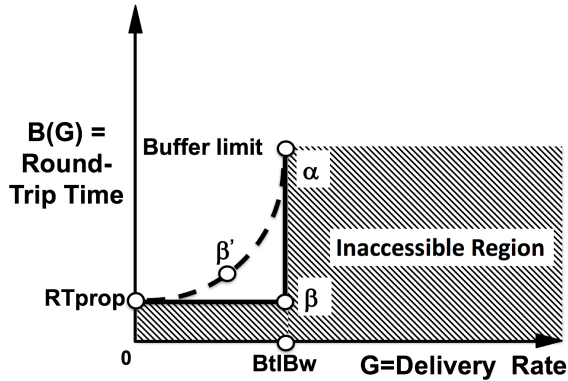
Figure 17: Comparing BBR ( \beta ), TCP ( \alpha ) and Power ( \beta' )
