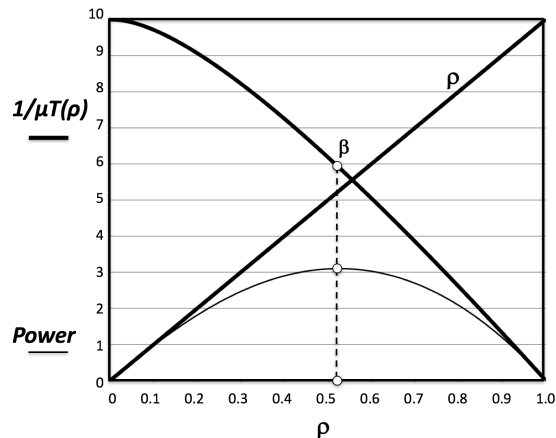
Figure 12: Optimality for the Queueing System E_2/M/1
