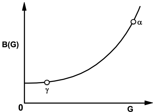
Figure 7: Stochastic Systems.
