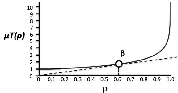
Figure 16: The Finite Resource Queueing System
