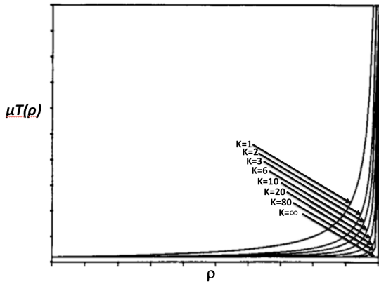
(a) Limiting Behavior \rightarrow D/D/1 .
