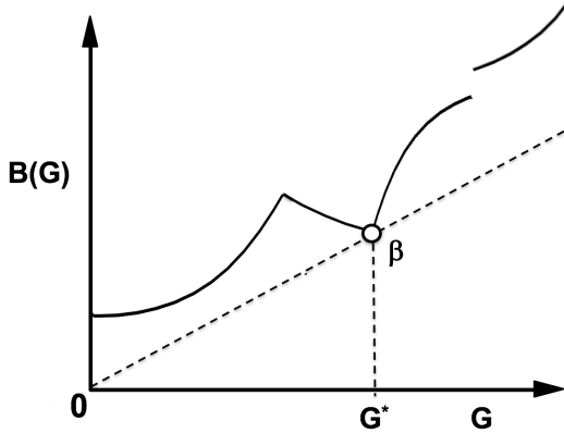
(b) Non-differentiable, Non-convex, Discontinuous B(G) .
